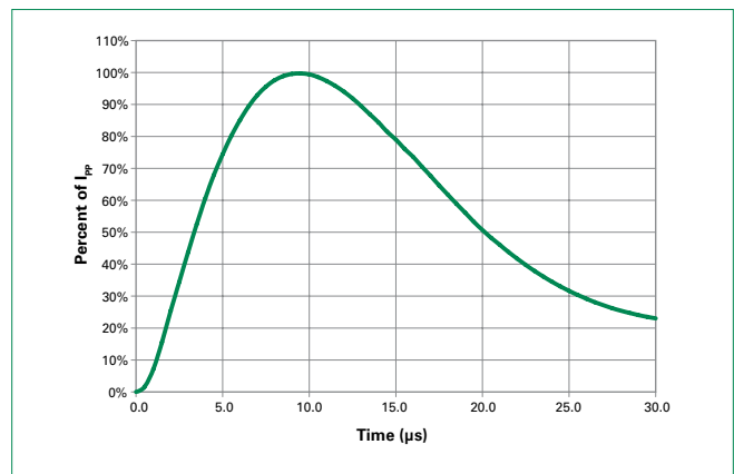
8/20 Pulse Waveform
