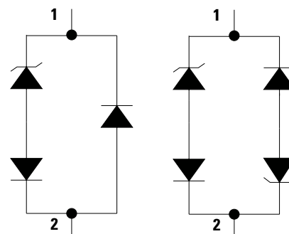
Unidirectional SP4020-01FTG
