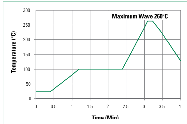
Figure 2 Lead-free Profile
