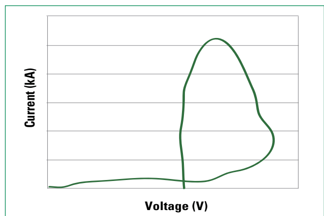
Figure 4 Surge Response
