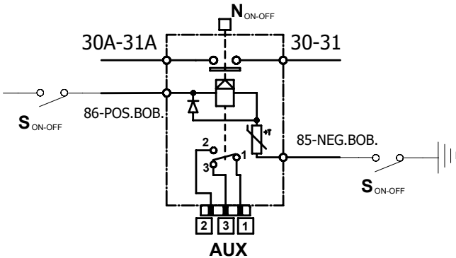
Fig. 1: Electrical diagram
