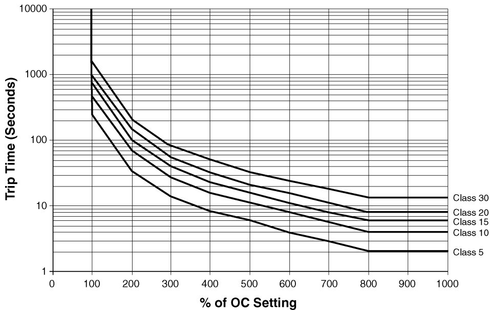
Figure 4: Overload Trip Curves
