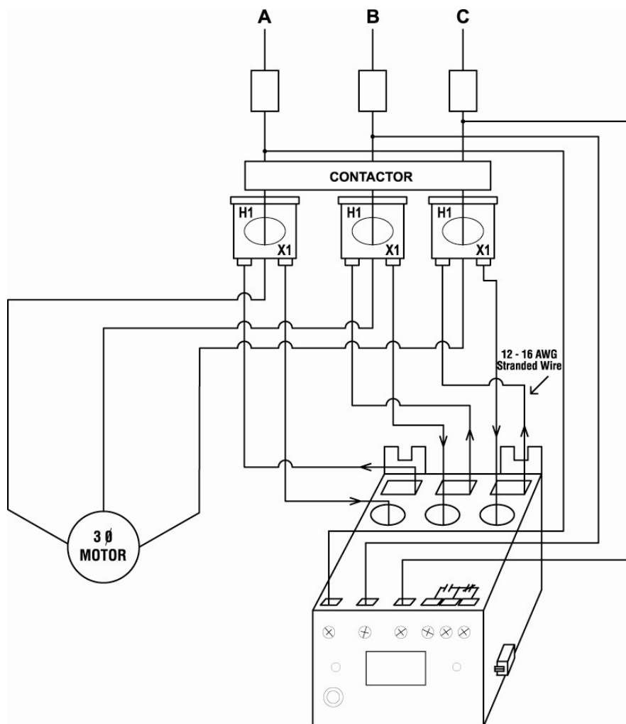
Figure 3: Typical Wiring Using External CTs 2
