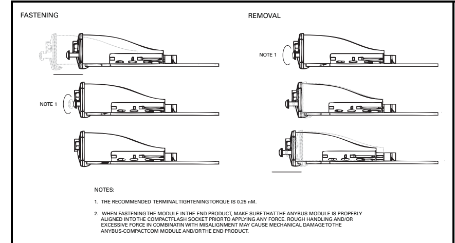
FIGURE 5. Anybus Communications Module Installation.
