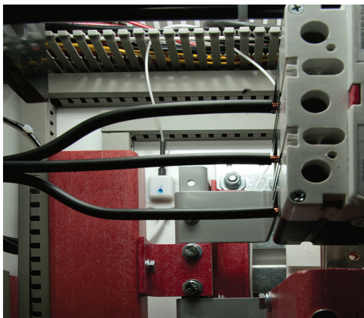
Example of appropriate fiber optic sensor installation.
