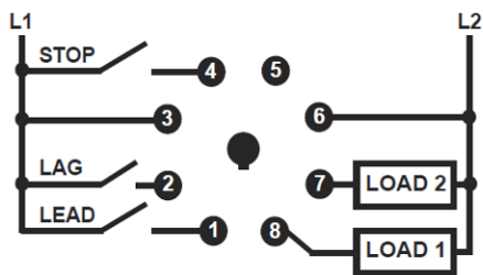
Figure 1: Pin-Out Diagram
