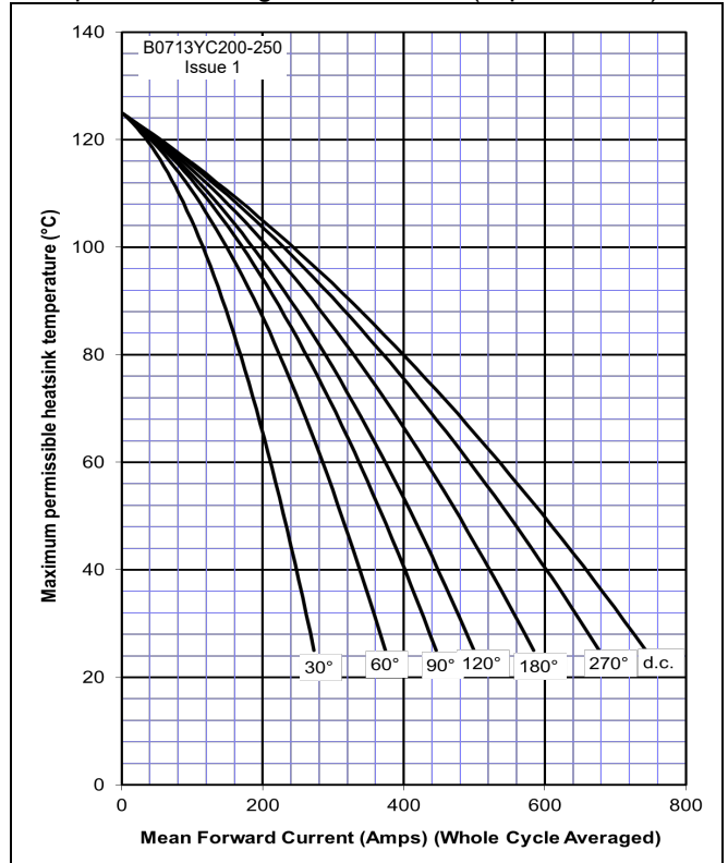
Figure 16 – On-state current vs. Heatsink temperature – Single Side Cooled (Square wave)
