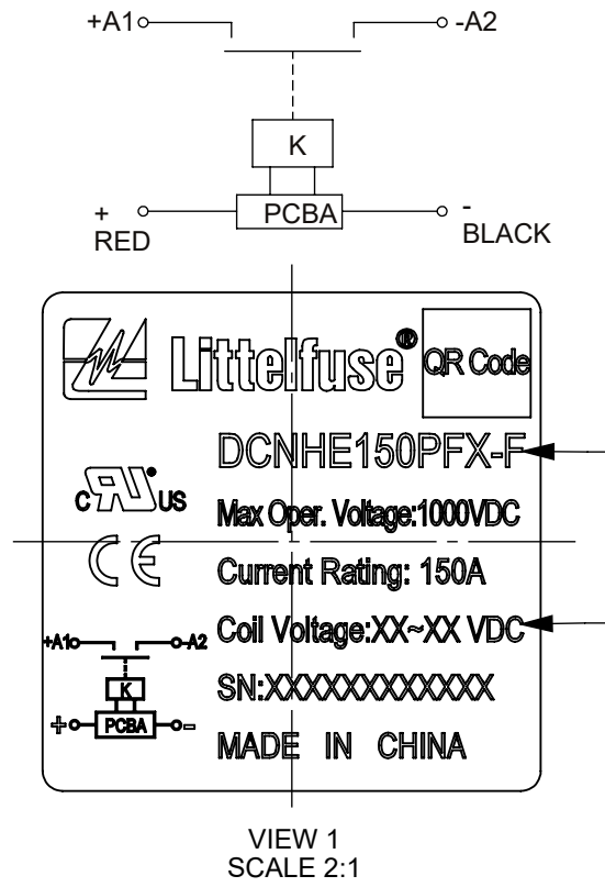
DCNHE150PF SERIES SCHEMATIC CIRCUIT DIAGRAM
