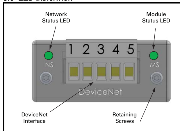
FIGURE 1. LED Indicators.
