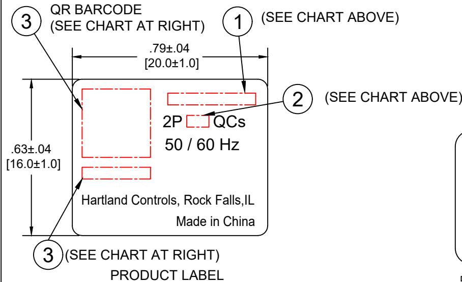
PRODUCT LABEL
