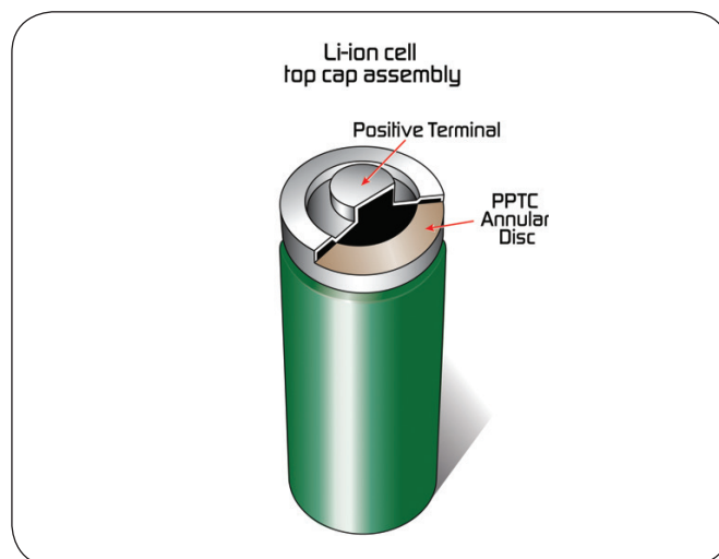
Figure 1. PPTC annular disc devices work in conjunction with other safety devices.
