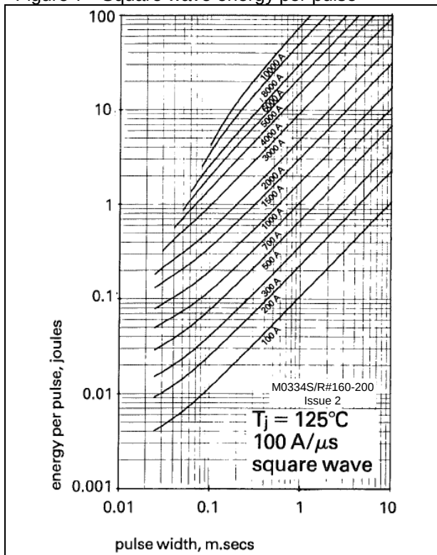
Figure 7 - Square wave energy per pulse
