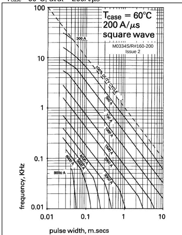
Figure 11 - Square wave frequency vs. pulse width, T_{case} = 60^{\circ}C , di/dt = 200A/\mu s
