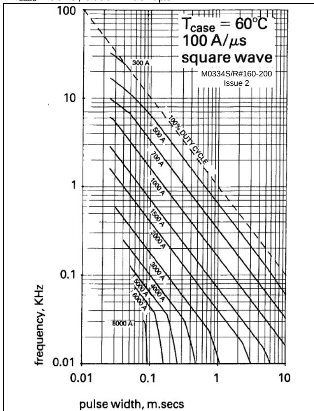
Figure 9 - Square wave frequency vs. pulse width, T_{case} = 60^{\circ}C , di/dt = 100A/\mu s
