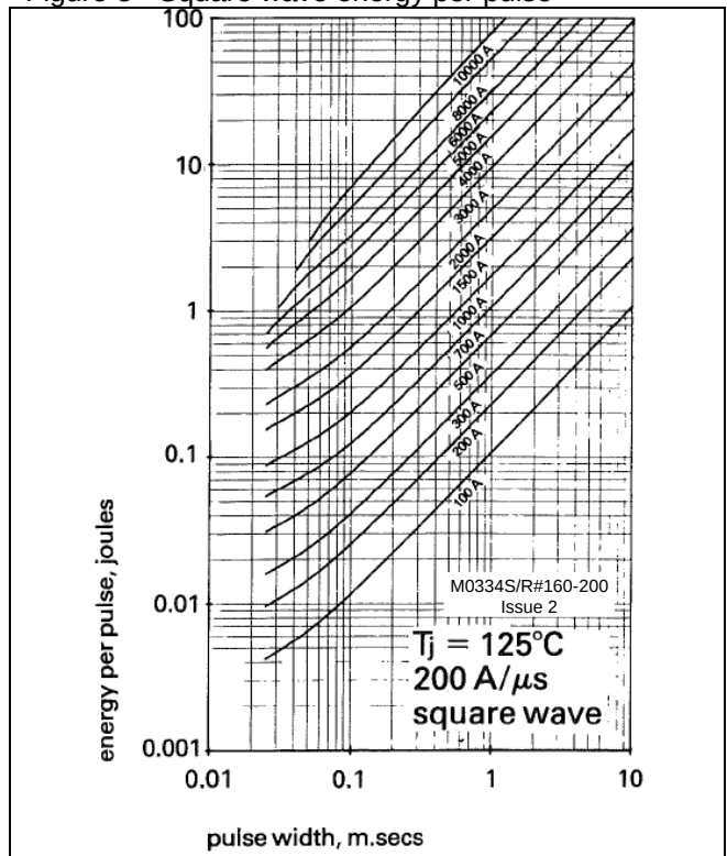
Figure 8 - Square wave energy per pulse
