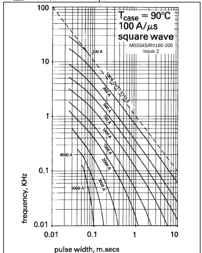
Figure 10 - Square wave frequency vs. pulse width, T_{case} = 90^{\circ}C , di/dt = 100A/\mu s
