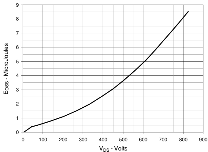
Fig. 11. Output Capacitance Stored Energy
