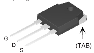
TO-3P (IXTQ)
