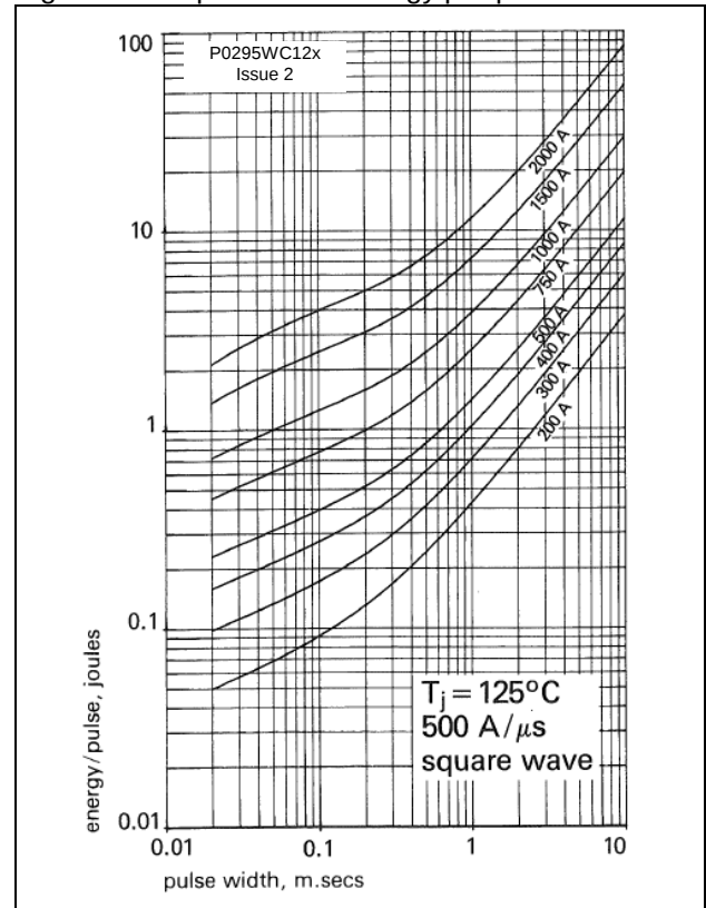
Figure 14 - Square wave energy per pulse
