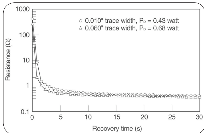
Figure 5. Typical resistance vs. time for varying trace widths for a surface-mount device.
