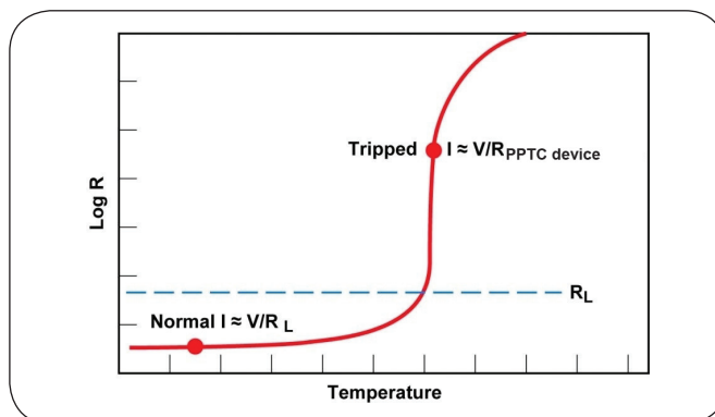
Figure 3. Typical operating curve for a PPTC device.
