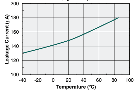
Typical Leakage Current vs. Temperature (V L =400V p )
