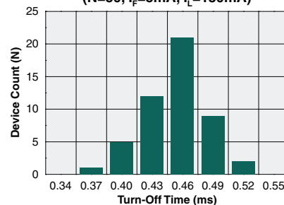
Typical Turn-Off Time (N=50, I_F=5\text{mA} , I_L=130\text{mA} )
