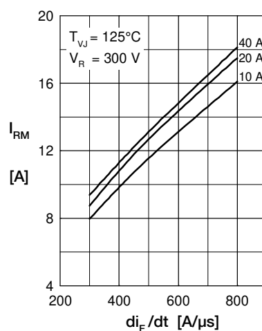
Fig. 3 Typ. peak reverse current I_{RM} versus di_F/dt
