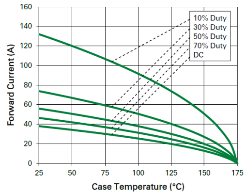
Figure 4: Current Derating
