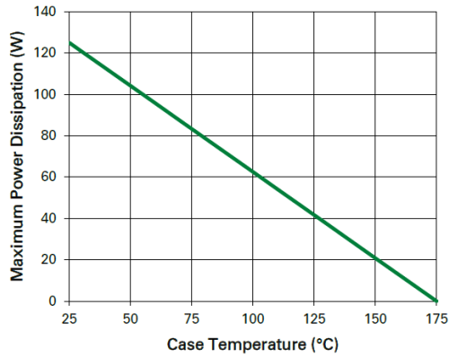
Figure 3: Power Derating
