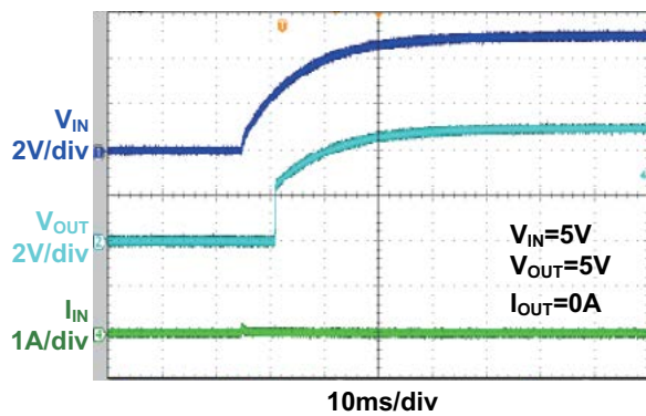
Figure 3 - V IN On (5V IN , I O = 0 A)
