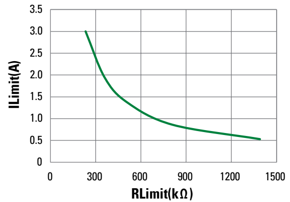
Figure 2 - RLimit vs. ILimit (5V IN Application)
