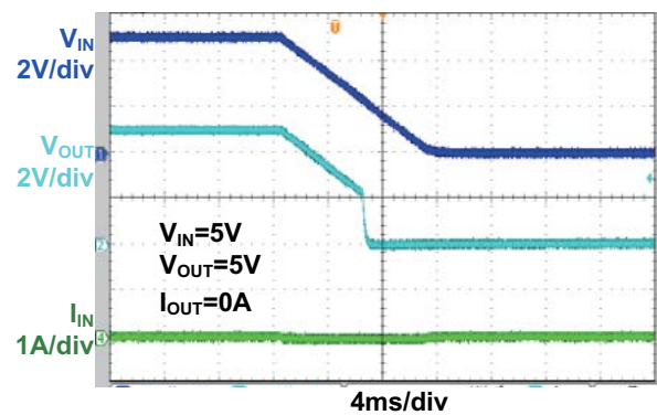
Figure 4 - V IN Off (5V IN , I O = 0 A)
