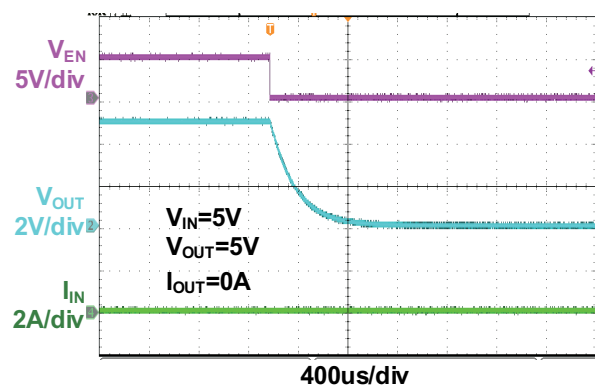
EN Power off ( I_{OUT} = 0 A )
