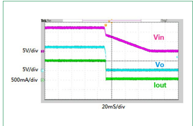
Figure 7. Shutdown (12V Mode, I_O=1A , C_{SS}=100nF )
