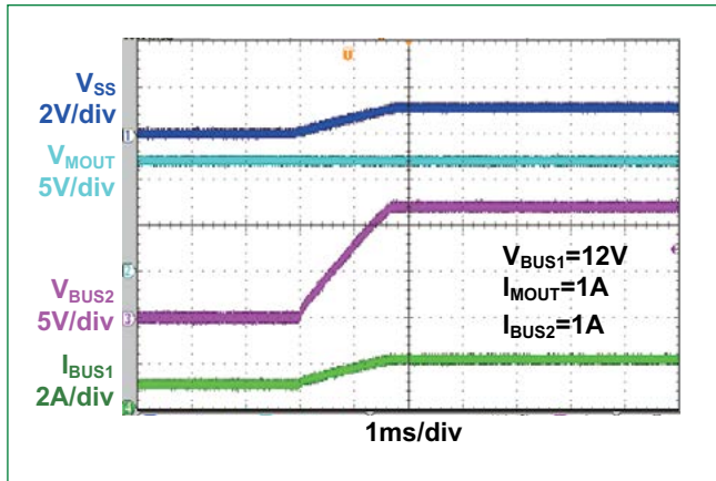
Figure 3. Programmable Soft-Start Time ( V_{BUS1} on, C_{SS}=10nF )
