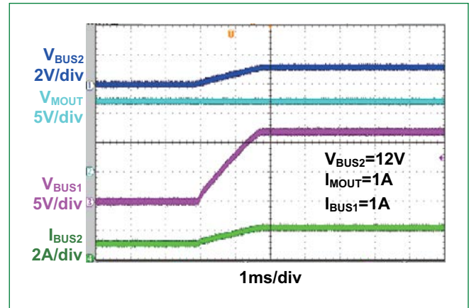
Figure 4. Programmable Soft-Start Time ( V_{BUS2} on, C_{SS}=10nF )
