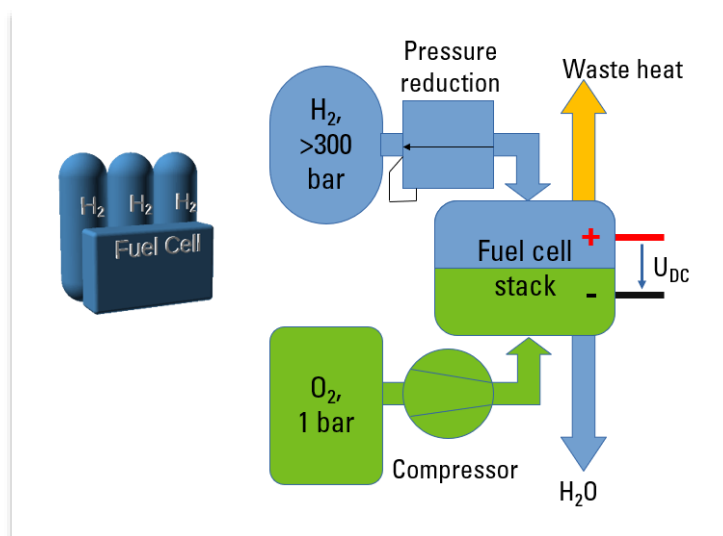
Figure 7. Fuel-cell-based Energy Conversion System
