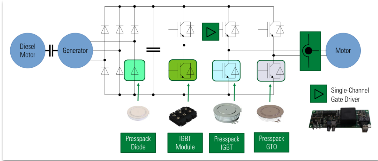
Figure 21. High-power Drive Train in Mobile MW Applications
