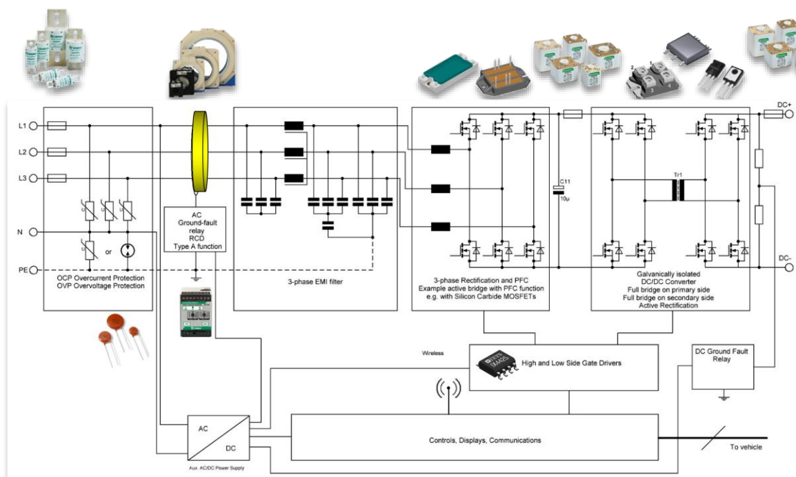
Figure 11. Bidirectional Charger Schematic and Suitable Components
