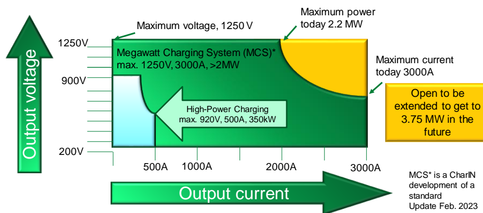
Figure 17: Comparing the Operating Area of High-power Passenger Car and Commercial Vehicle Chargers
