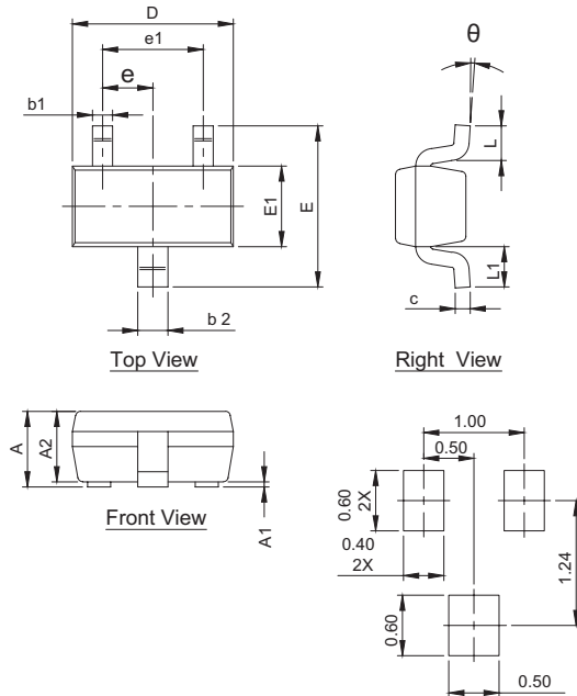
Recommended Soldering Pattern (unit :mm)
