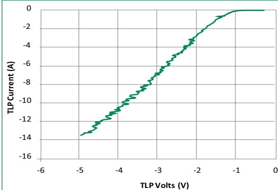
Negative Transmission Line Pulsing (TLP) Plot (Pin 2, 3, 4 to GND )
