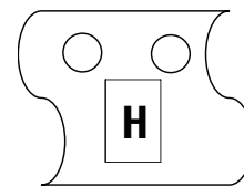
Component Orientation in Tape
