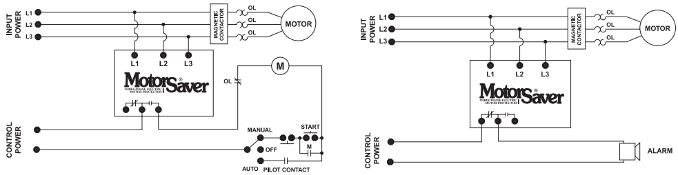
(A) To control a motor: Connect the normally open contact in series with the magnetic coil of the motor starter as shown. (B) To sound an alarm: Connect the normally closed contact in series with the alarm as shown.
