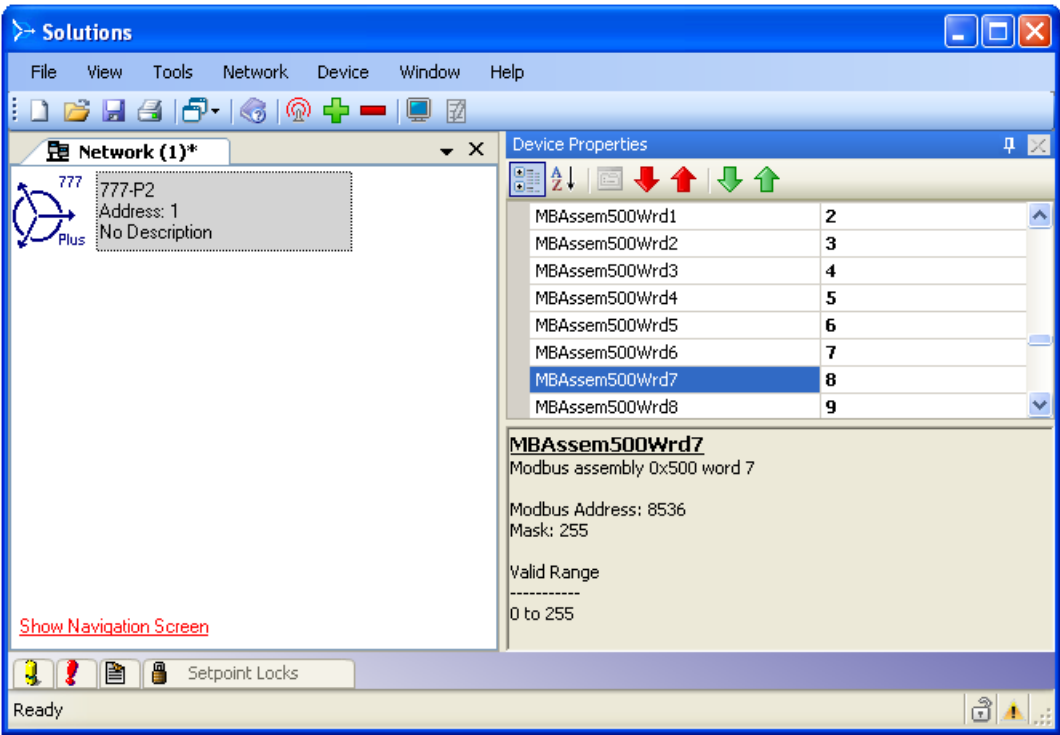
Figure 1 - Modbus Assembly
