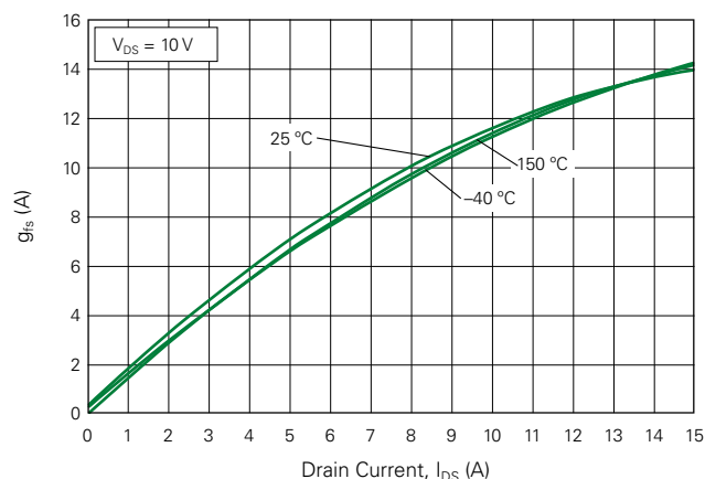
Fig. 2. Typical Transconductance
