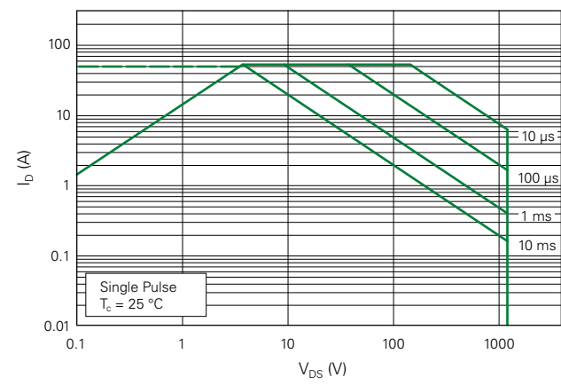
Fig. 26. Maximum Safe Operating Area ( T_c = 25\text{ }^{\circ}\text{C} )
