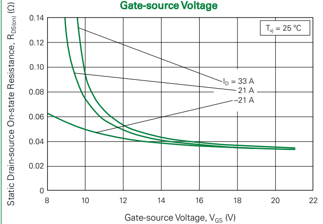
Fig. 8. Typical Drain-source On-state Resistance vs. Gate-source Voltage
