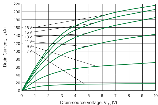
Fig. 3. Typical Output Characteristics @ T_J = 25 °C
