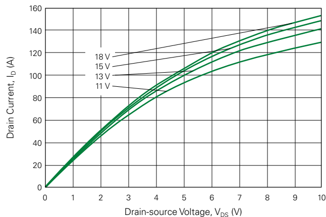
Fig. 4. Typical Output Characteristics @ T_J = 150 °C
