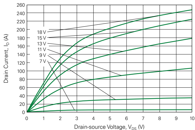
Fig. 5. Typical Output Characteristics @ T_J = -40 °C
