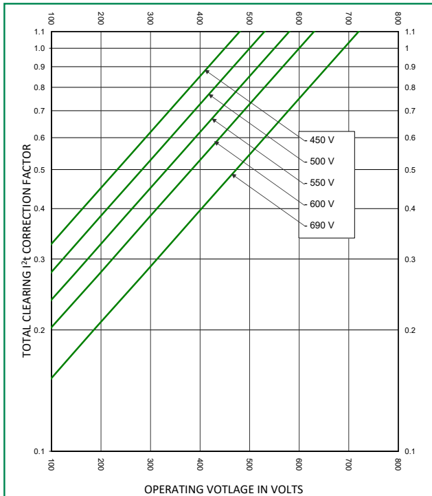
Total Clearing I^2t Correction Factor Curve (30, 31, 32 and 33 Case Sizes)
