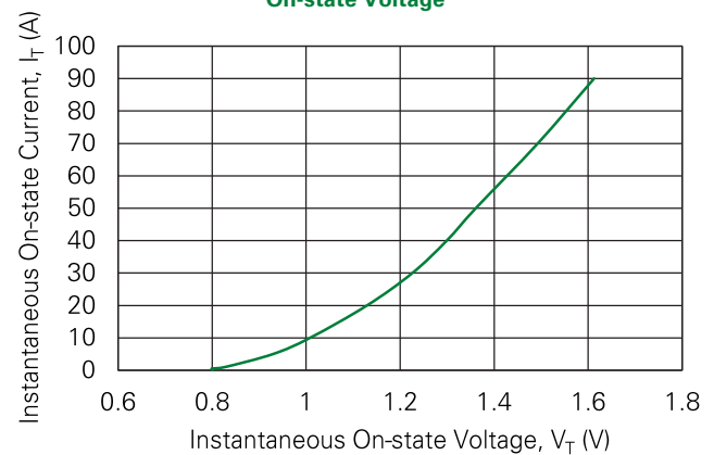
Fig. 6. Typical On-state Current vs. On-state Voltage
