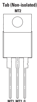
TO-220 (R-Package)
