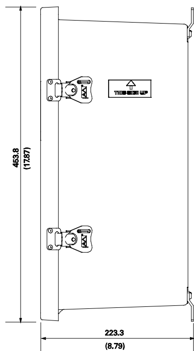
SIDE
