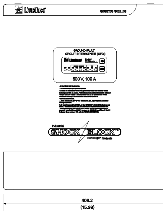
FRONT
