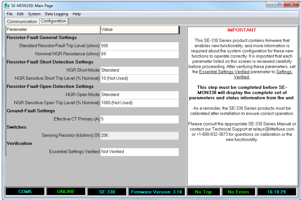
FIGURE 35. Initial Configuration Tab
